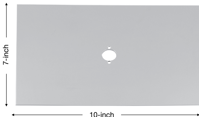
¾-inch Eurotherm Valve 7x10-inch
