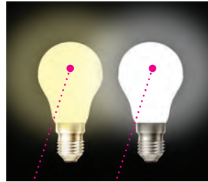
2700 Kelvin 4000 Kelvin
