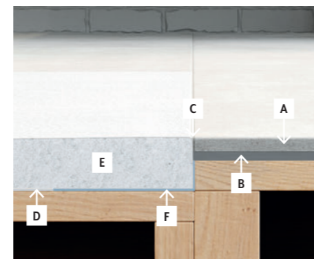
Recessed floor installation
