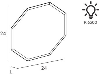
LED MIRROR
